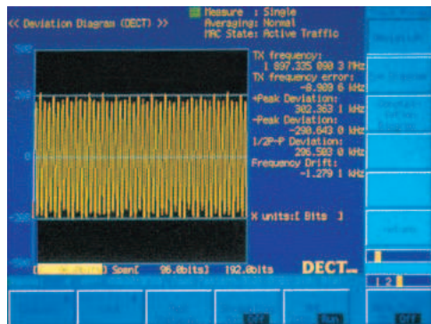
Example of transmitter modulation (DECT)
