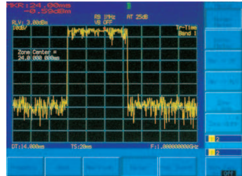
Burst wave measurement in time domain
