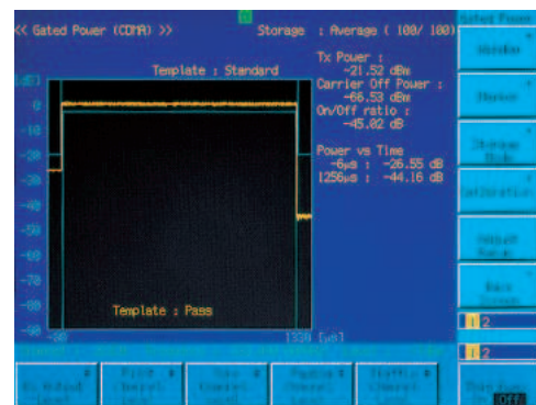
Gated output power measurement
