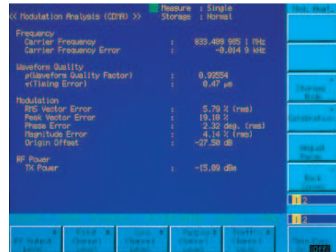
Waveform quality measurement
