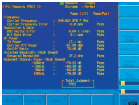
Example of linked send measurement items (PDC)
