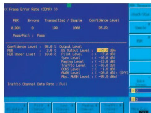
Frame error rate measurement
