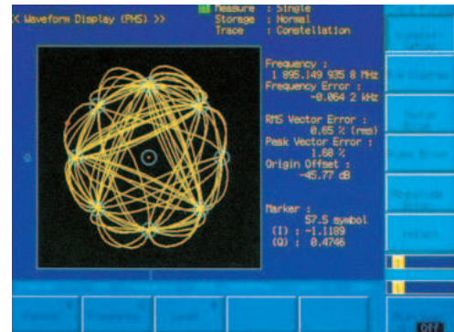
Example of constellation display (PHS)
