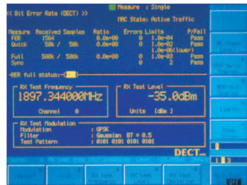
Example of bit error rate measurement (DECT)
