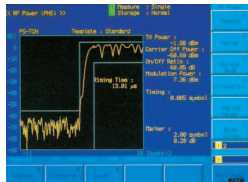
Example of burst rise characteristics (PHS)
